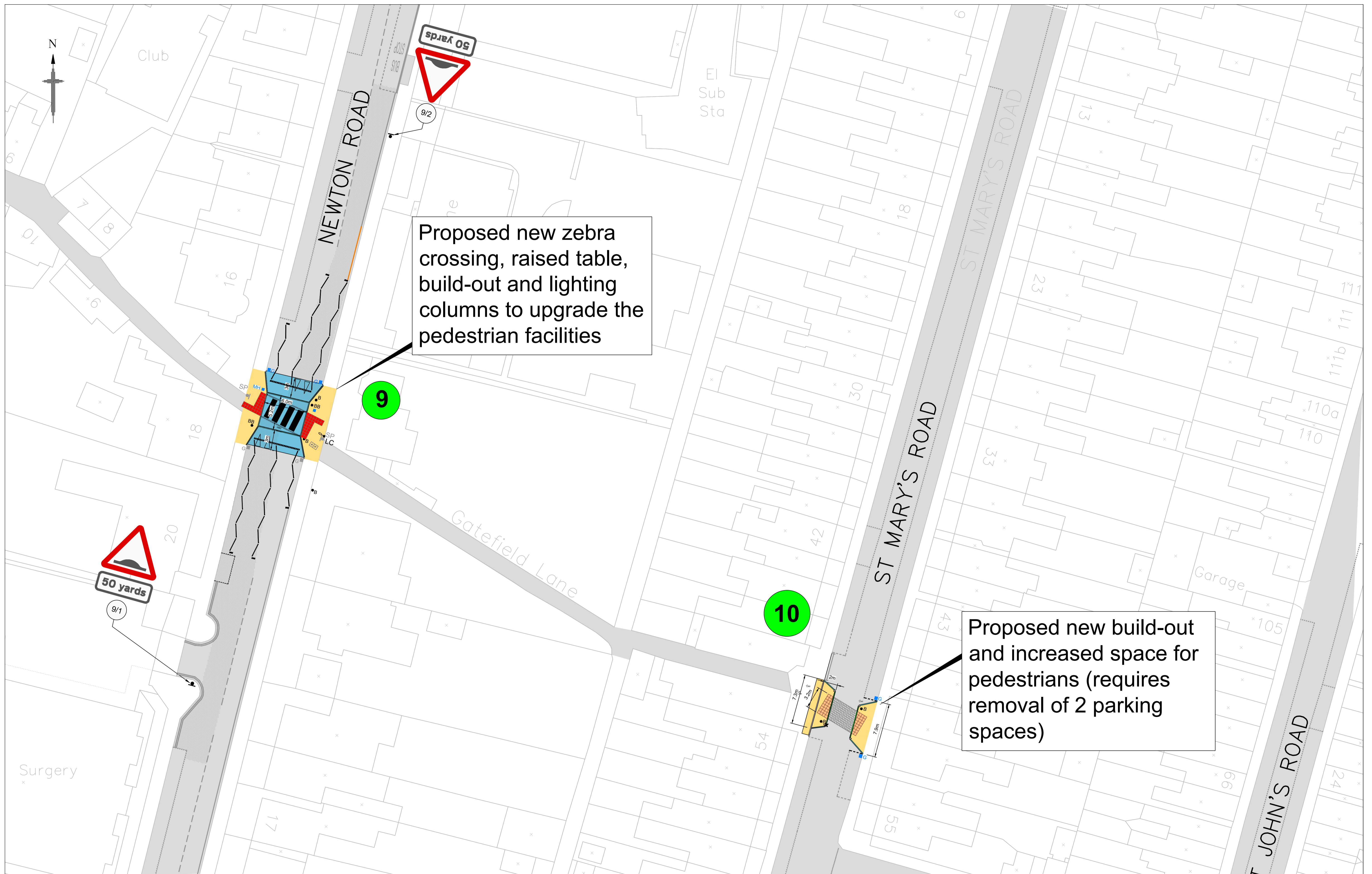
ACTIVE TRAVEL - FAVERSHAM PROPOSED CROSS TOWN WALKING ROUTE SCHEME 9 - NEWTON ROAD JUNCTION AND 10 - ST MARY'S ROAD JUNCTIONS WITH GATEFIELD LANE
