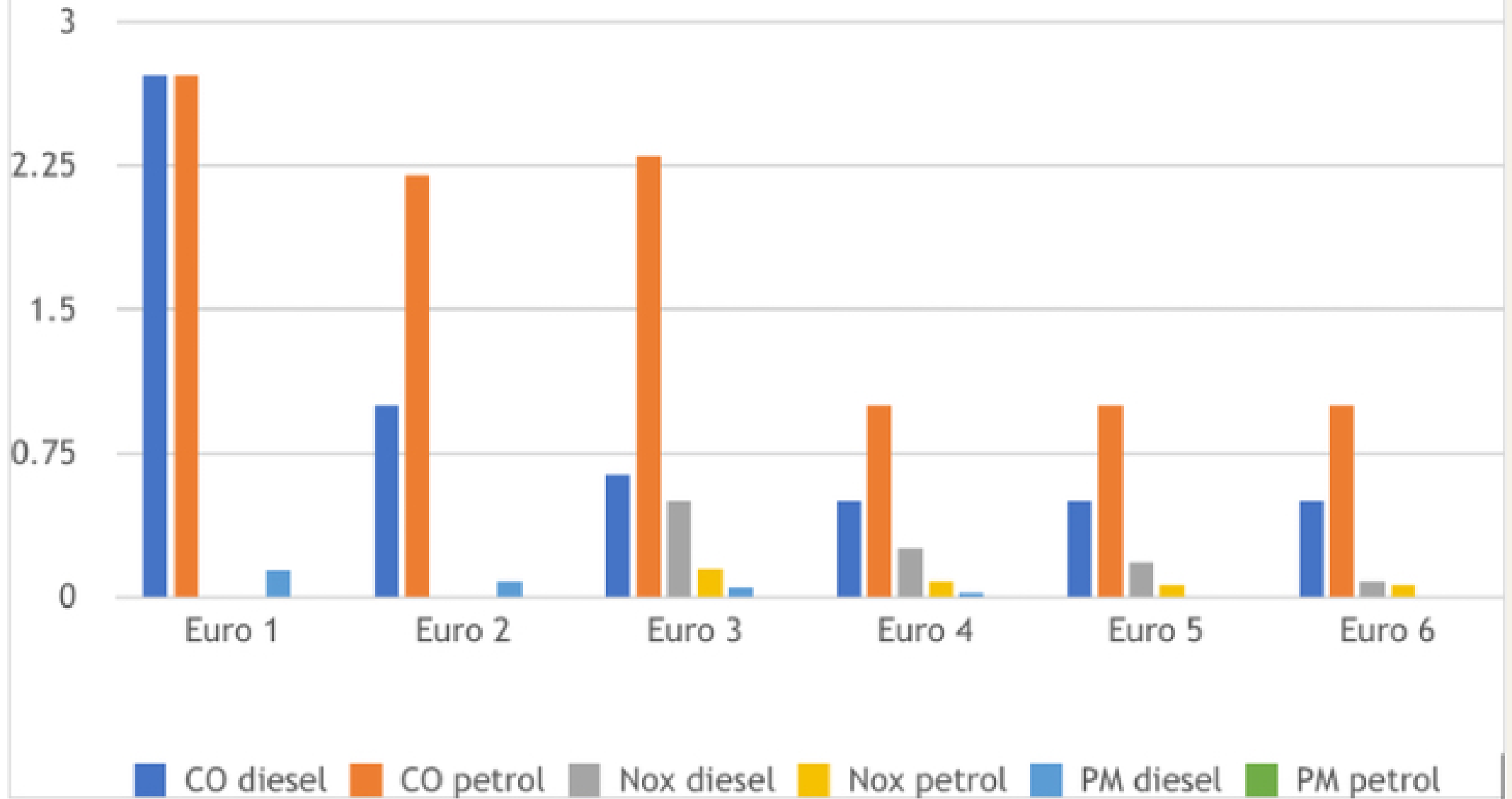
Fig. 1: EU Toxic Emissions limits - cars
